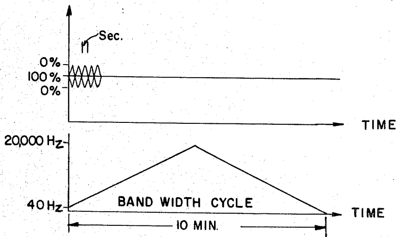
AUDIO SIGNAL AMPLITUDE MODULATION
